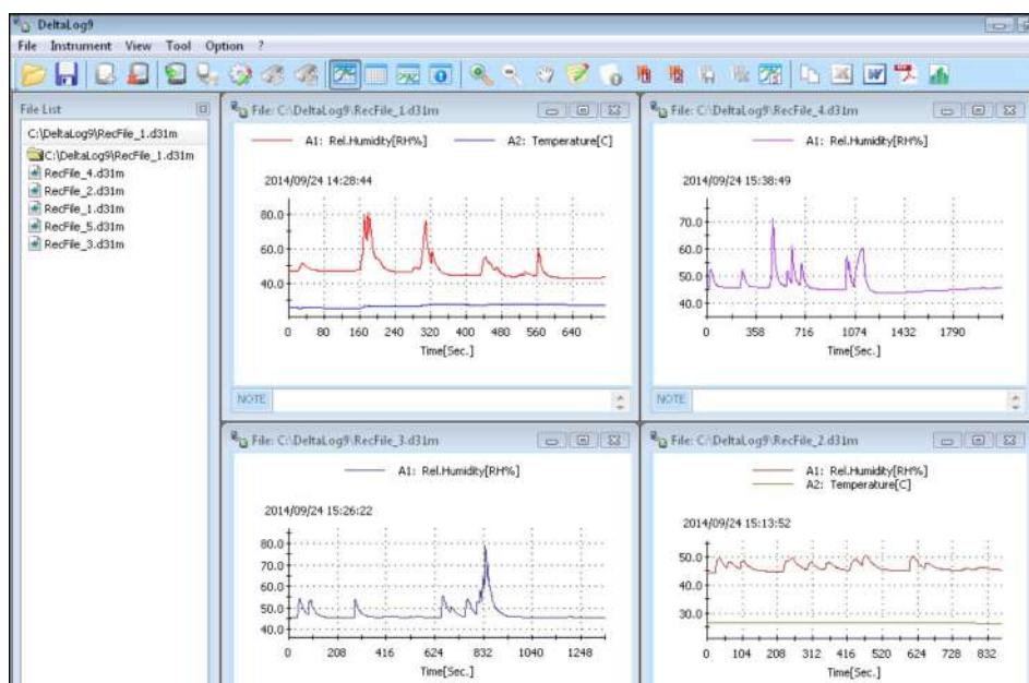
Software DeltaLog 9
